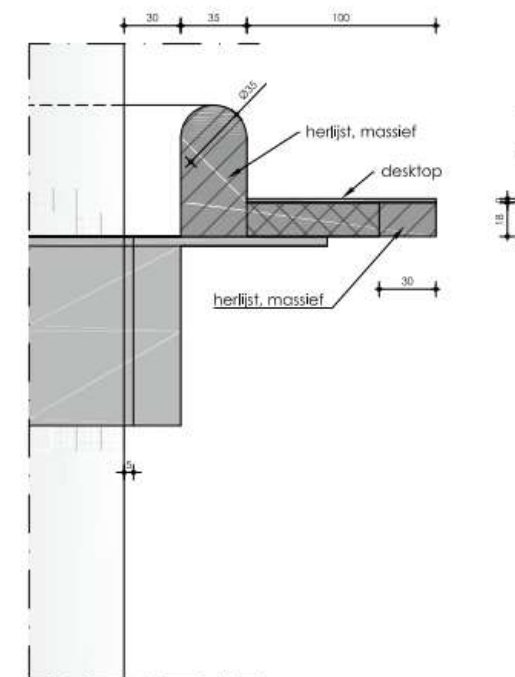
detail A 1:2
