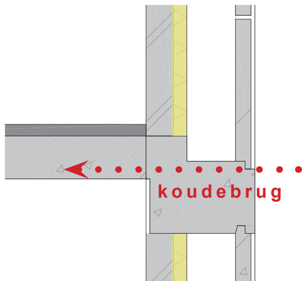
typical section, existing situation
