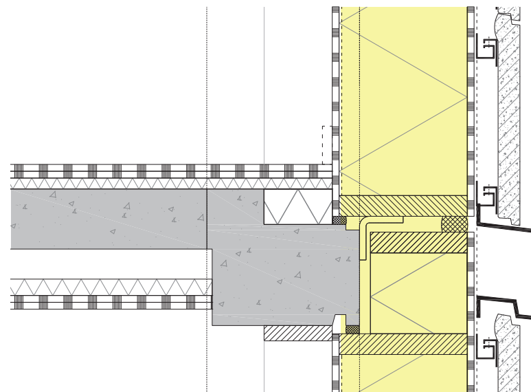
proposed typical section
