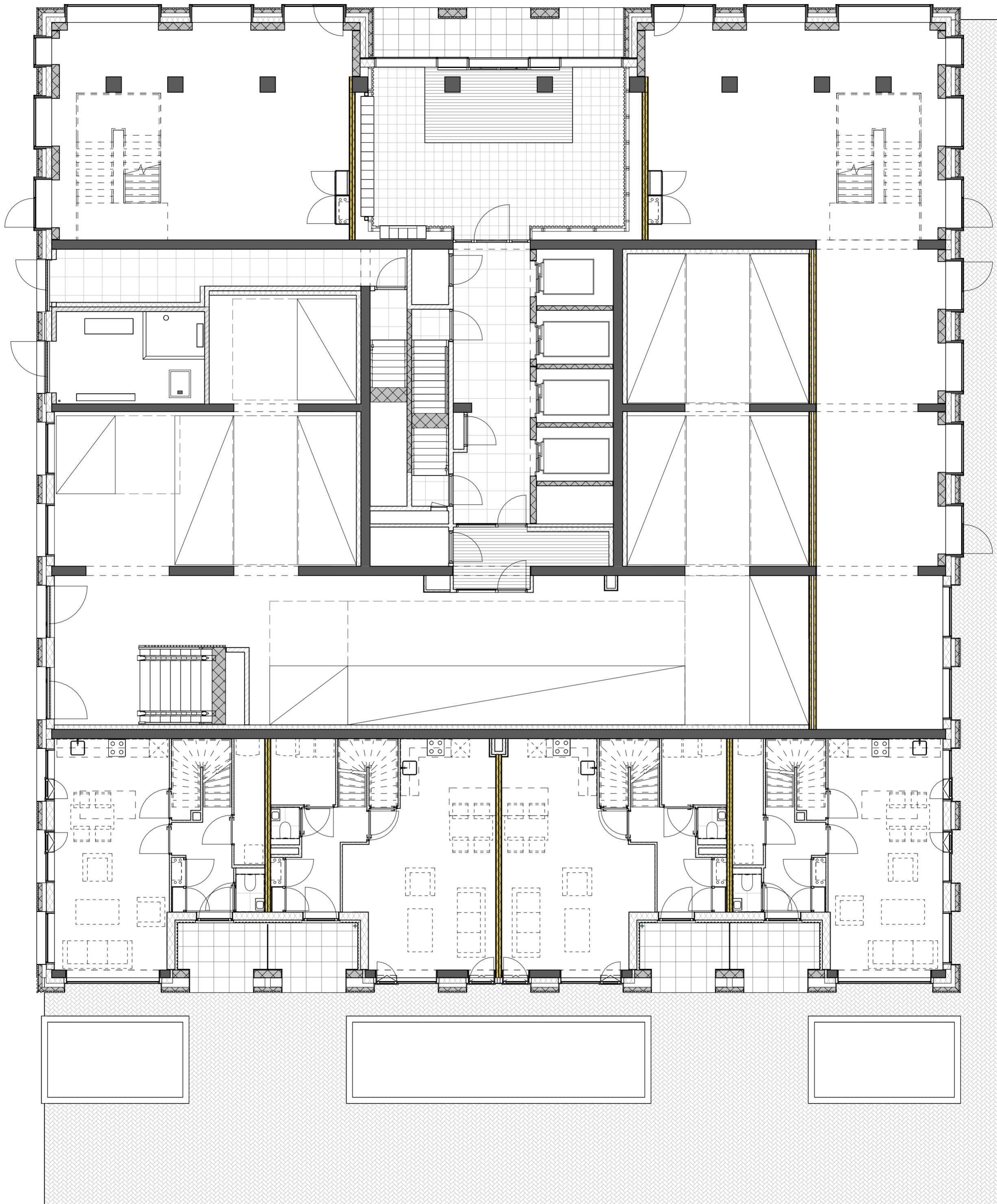
Begane grond, 1:100
