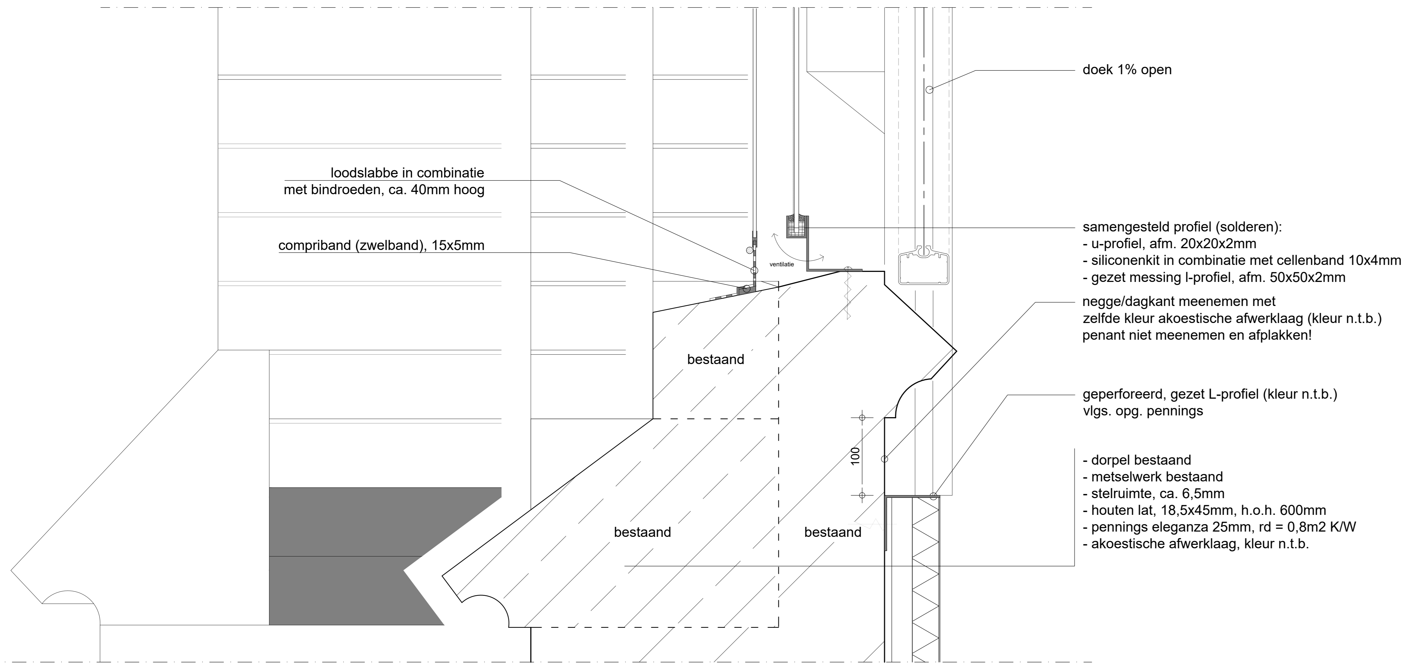
DETAIL V20
