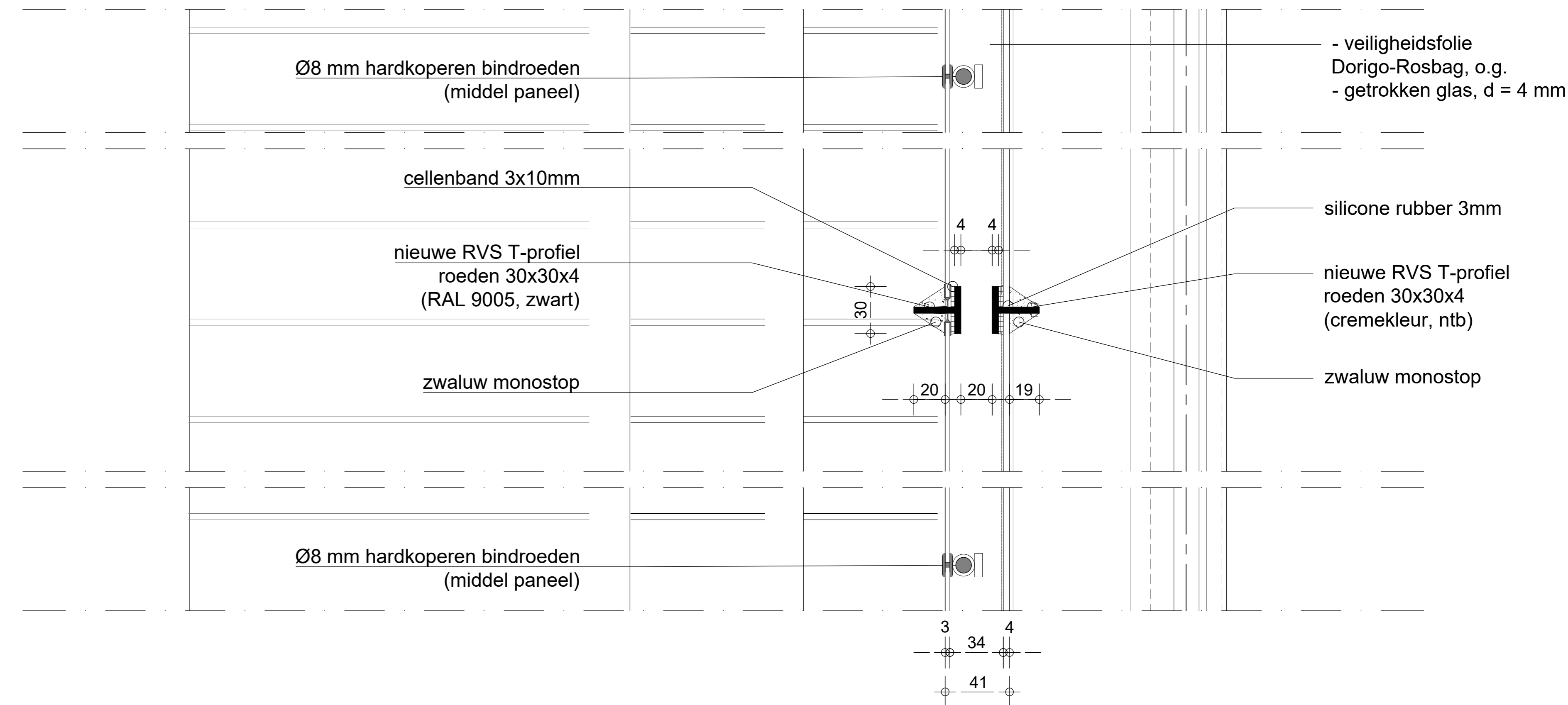
DETAIL V21
