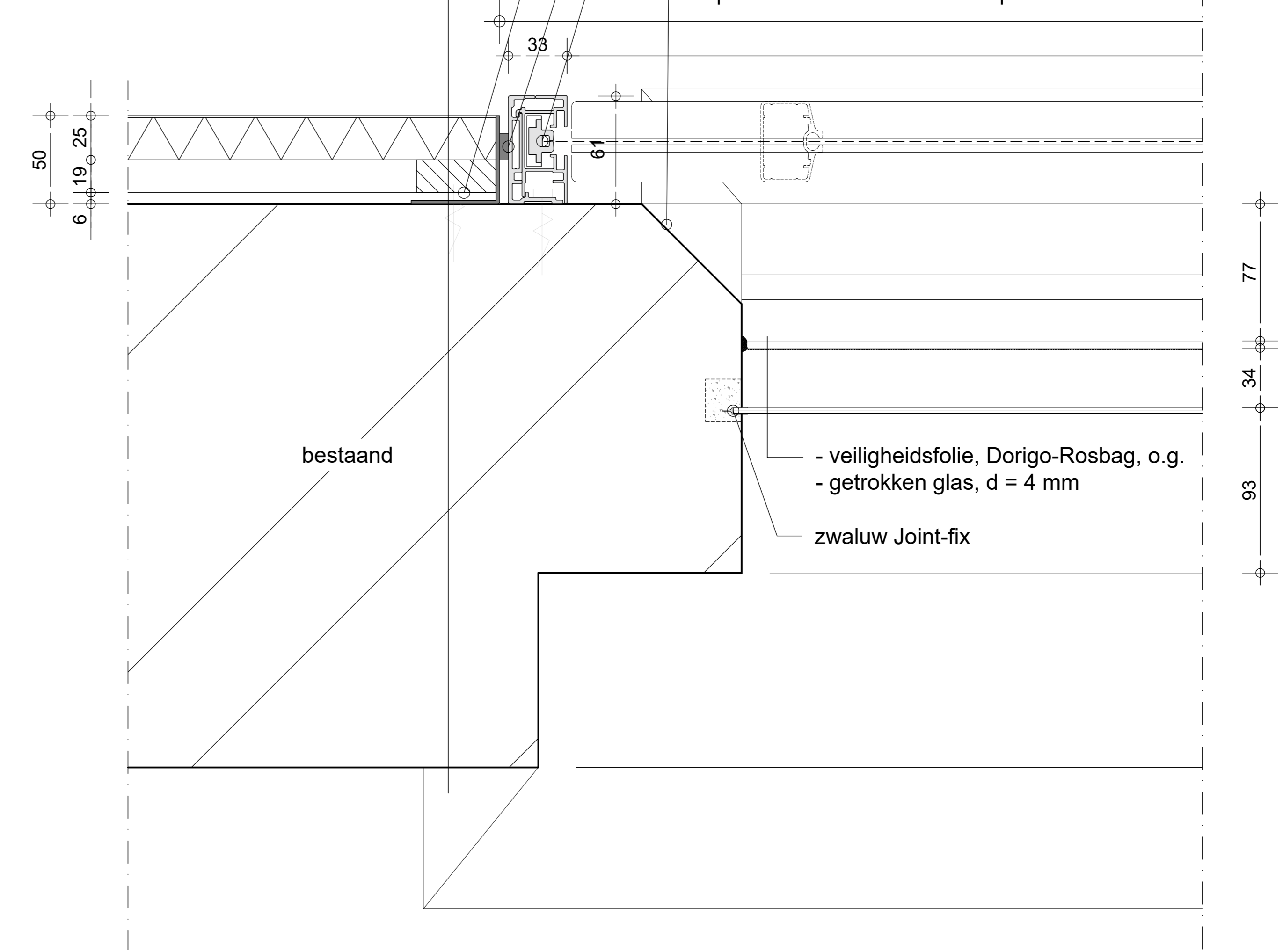
DETAIL H5
