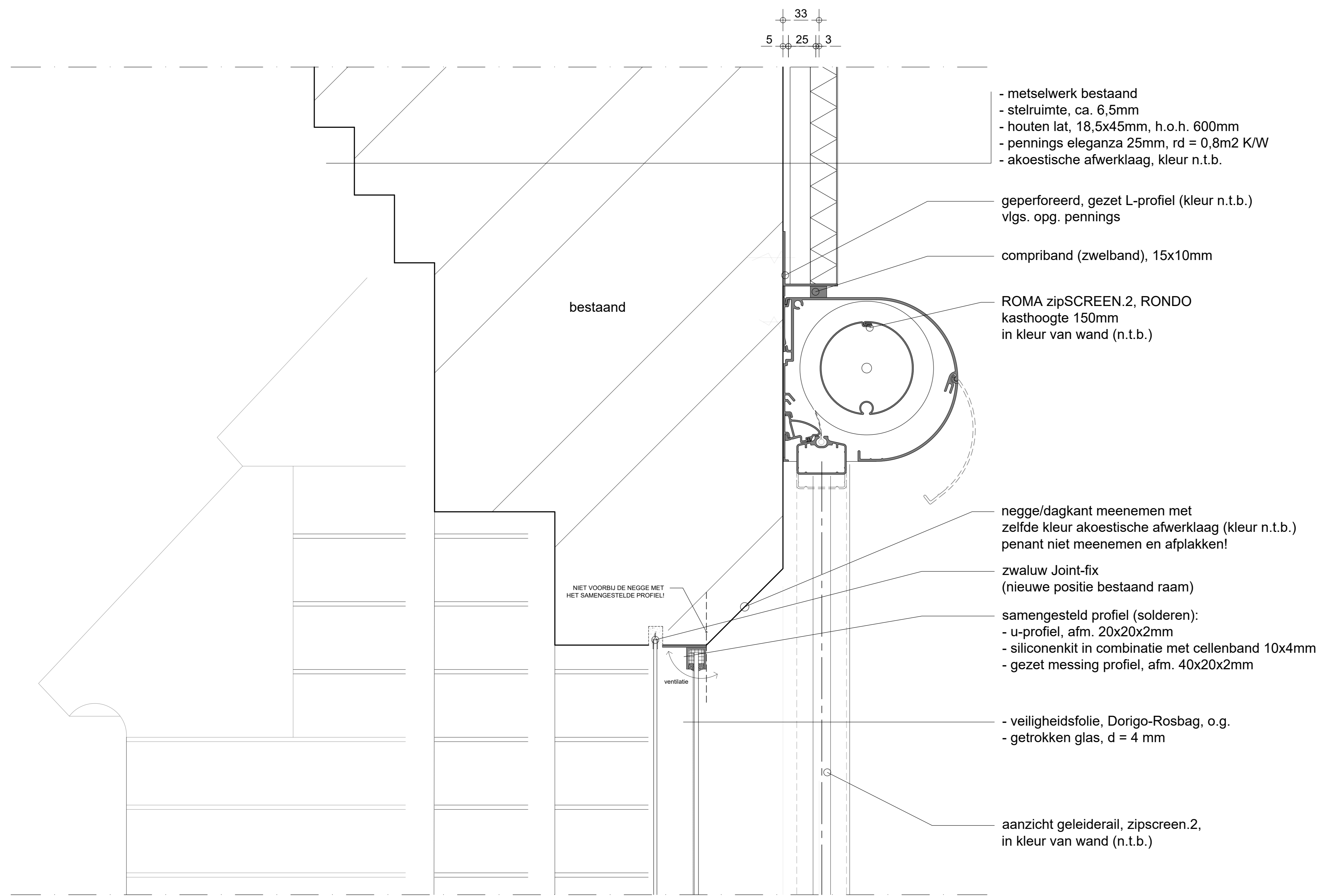
DETAIL V22
