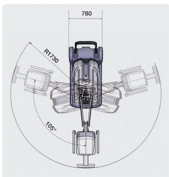
LIFT DIMENSION
