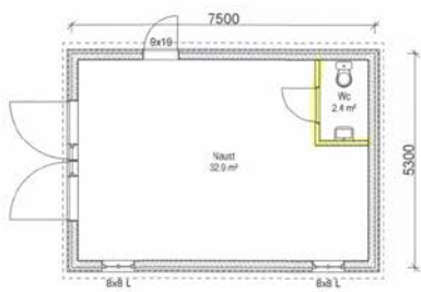
Plan naust
