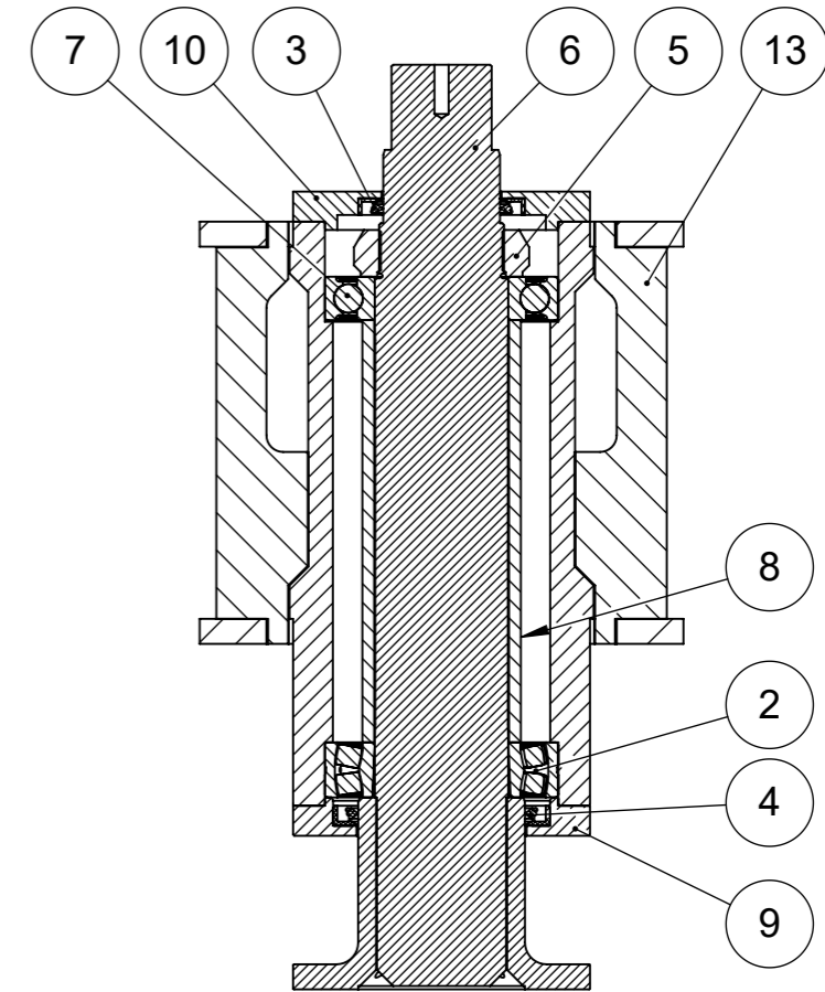
SECTION B-B
