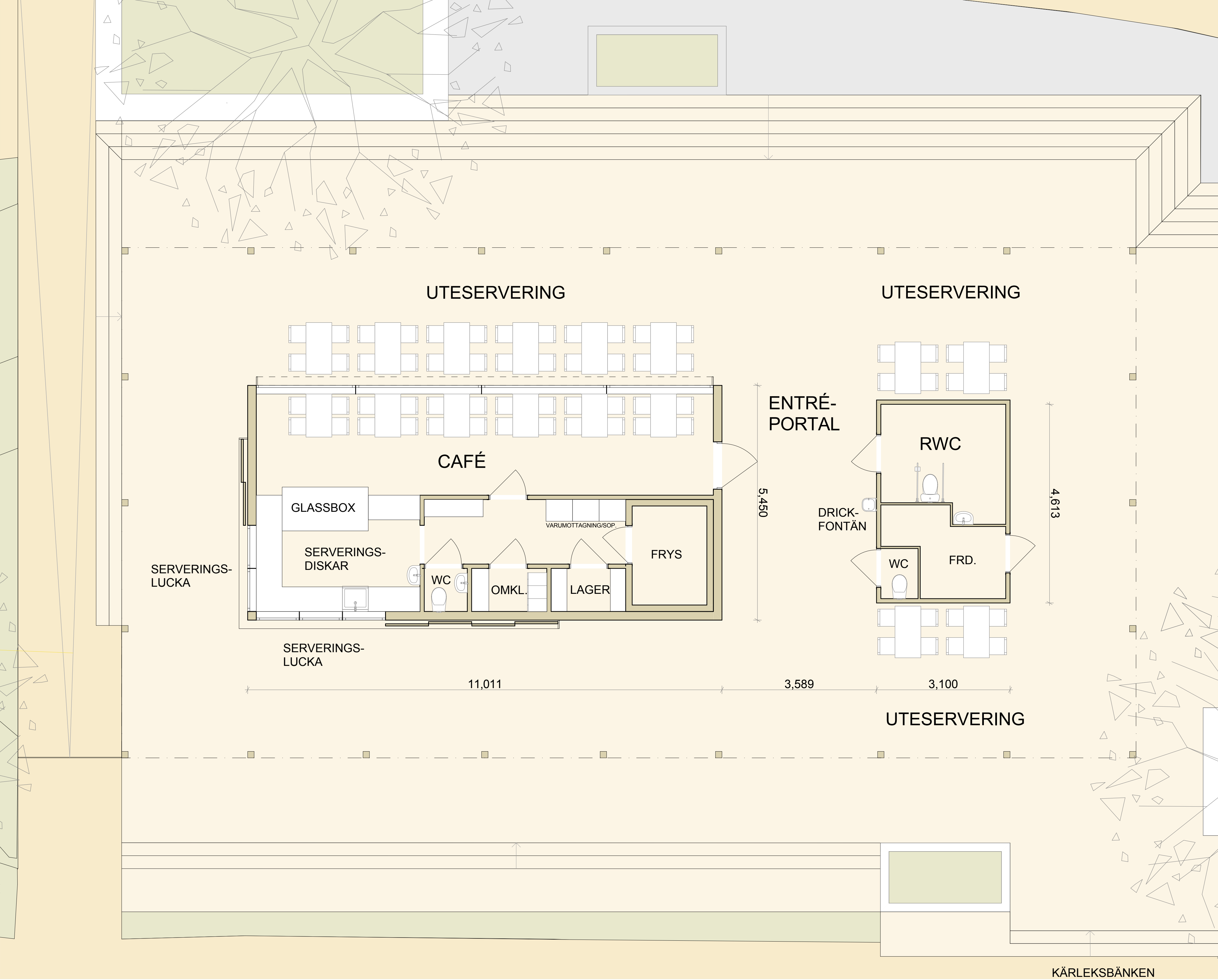
PLAN
