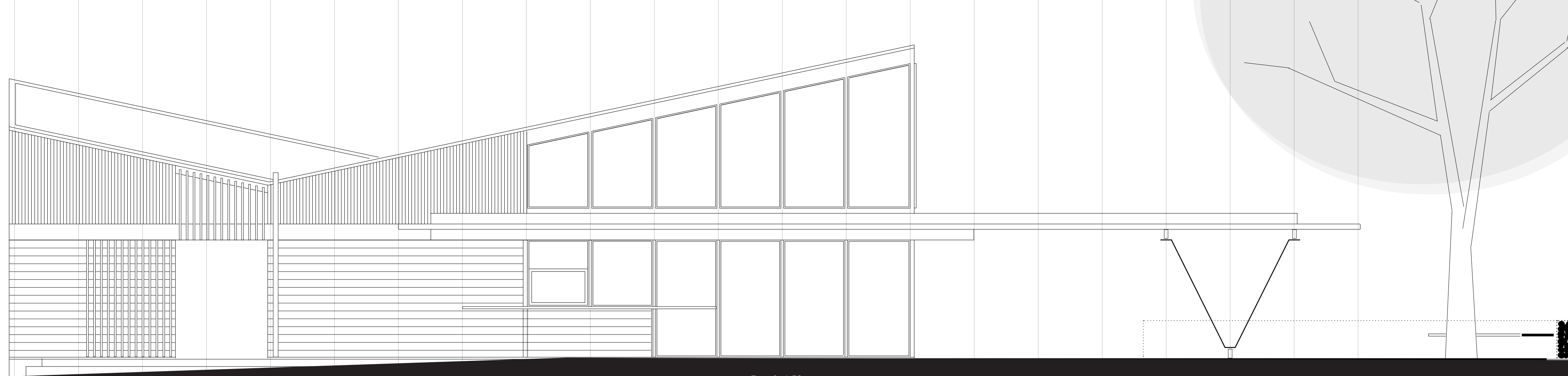
Facade 1:50
