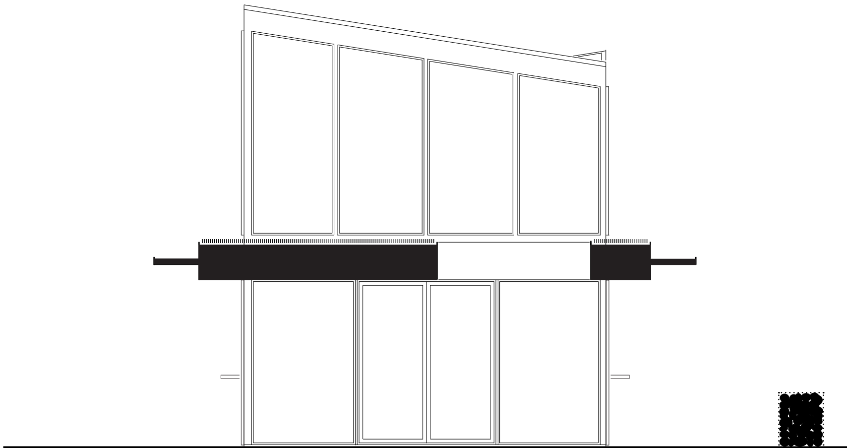
Facade 1:50
