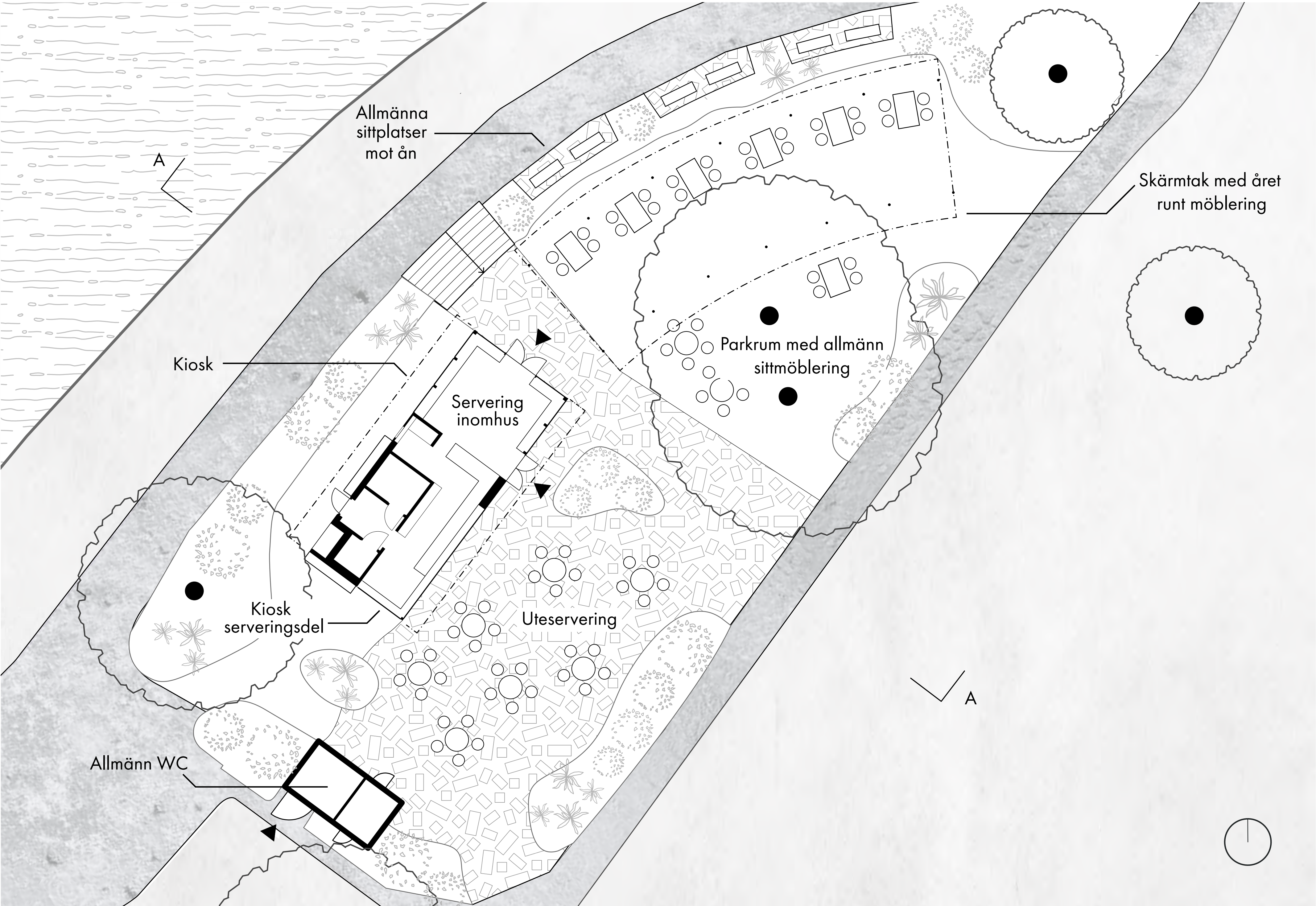
PLAN (1:100)
