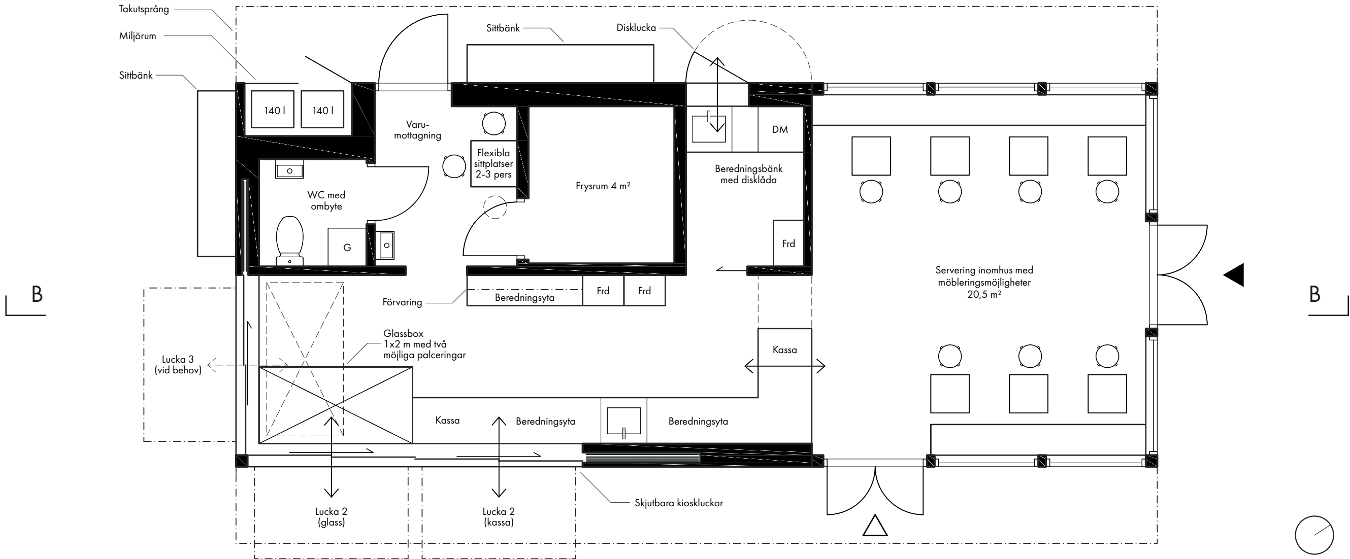
PLAN (1:50)
