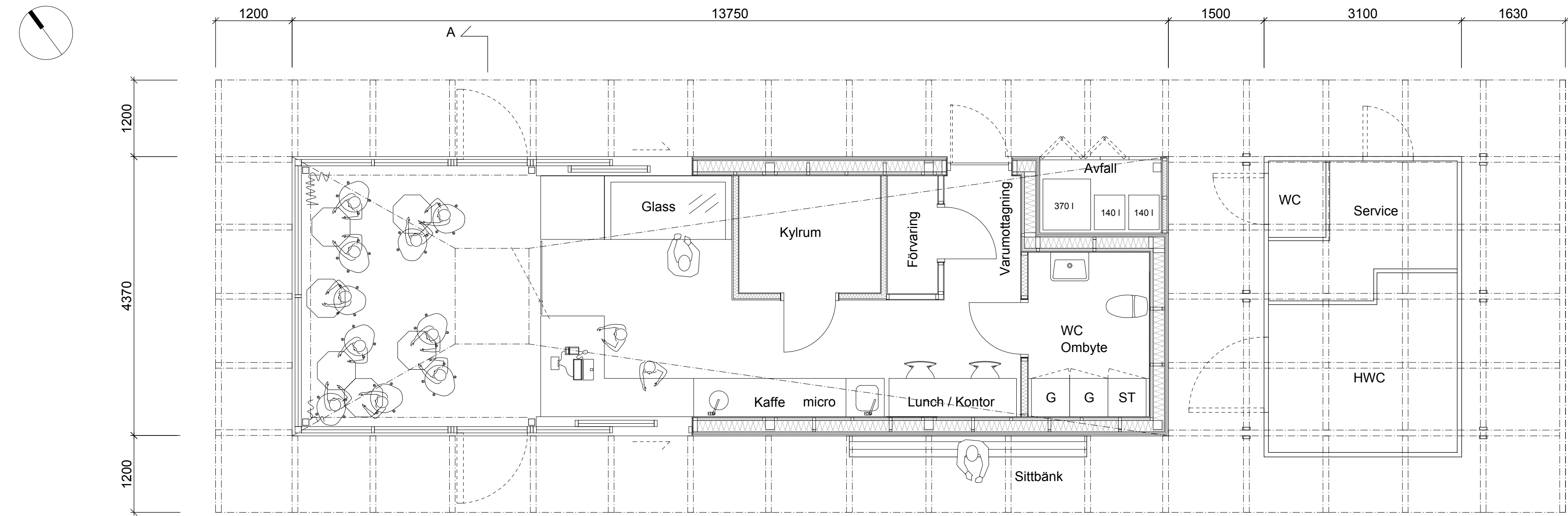
Plan 1:50. BTA 60 kvm
